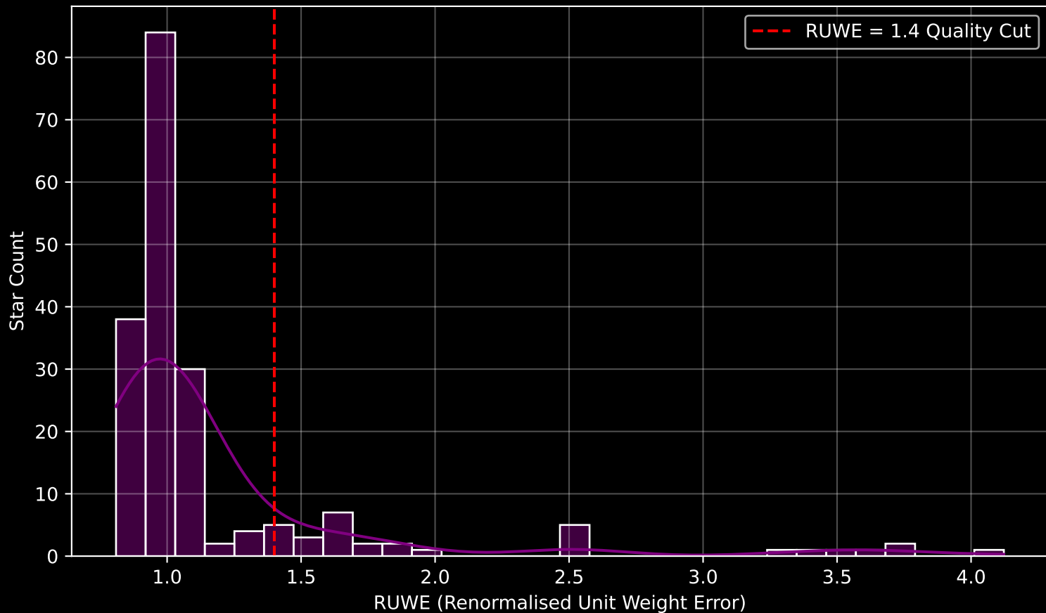
GAPOGEE DR17 Field [180-75] RUWE Distribution (n= 190)
