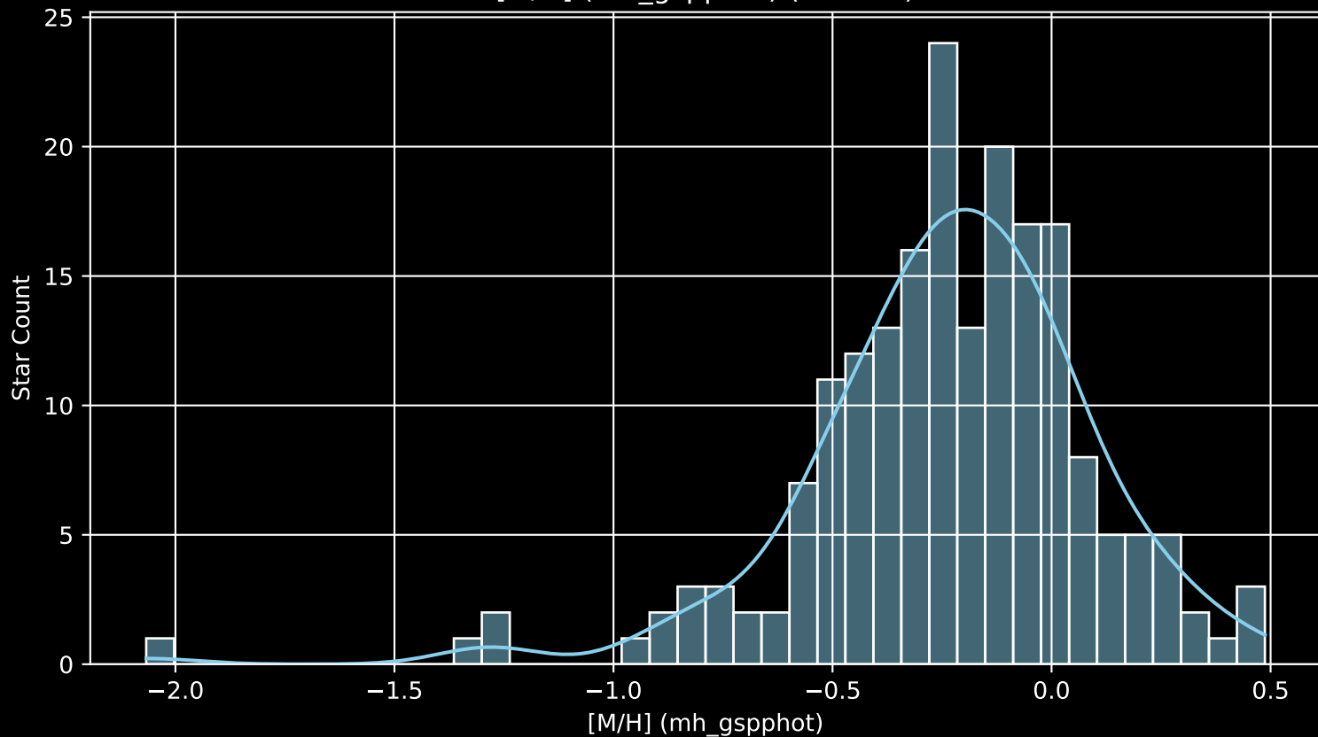
APOGEE DR17 Field: [180-75 [M/H] (mh_gspphot) (n= 196)
