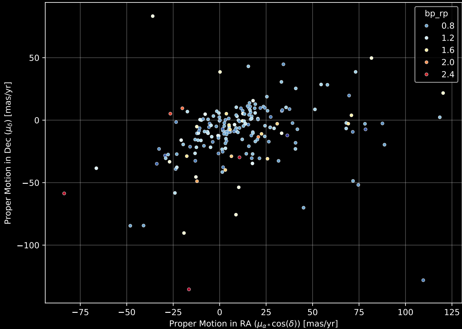
APOGEE DR17 Field: [180-75] Proper Motion Diagram (n= 199)
