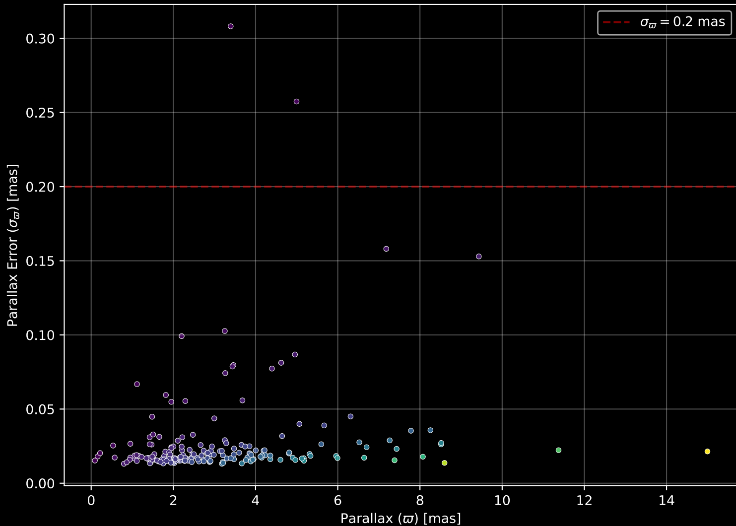
APOGEE DR17 Field: [180-75] Parallax Quality (n= 199)
